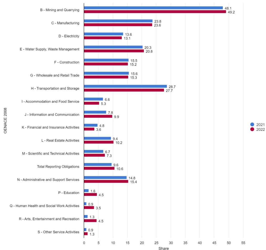
Enterprises obliged to report in Total Number of Enterprises - Share by Sections of OENACE 2008
